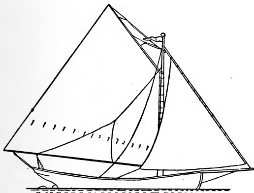
Jib and Mainsail Rig. Fig. 2.
